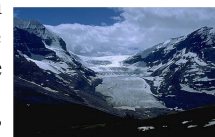
Athabasca Glacier
